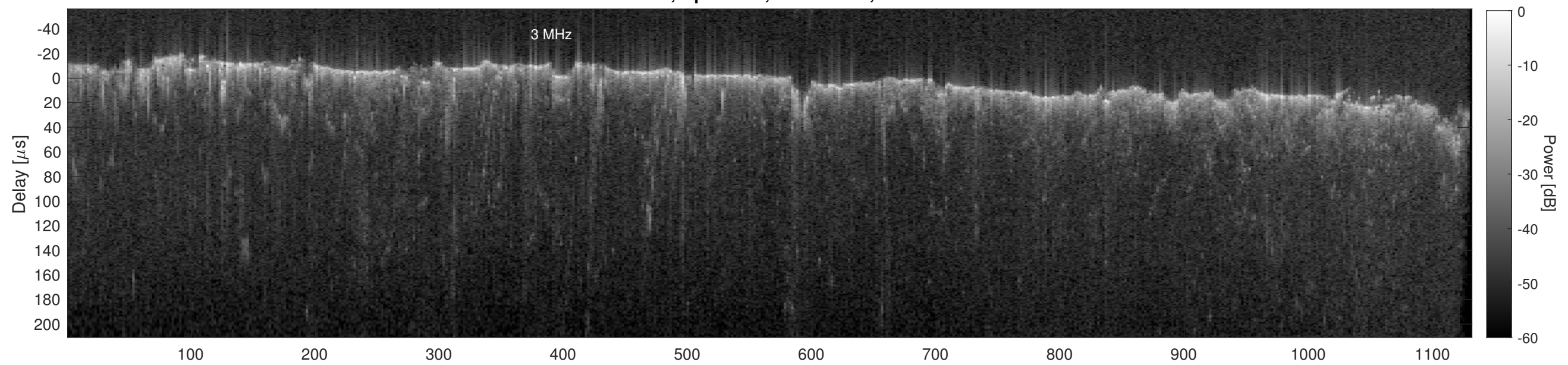
Orbit 20781, Cluttergram
