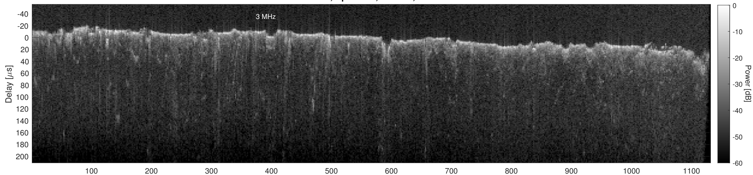
Orbit 20781, Cluttergram
