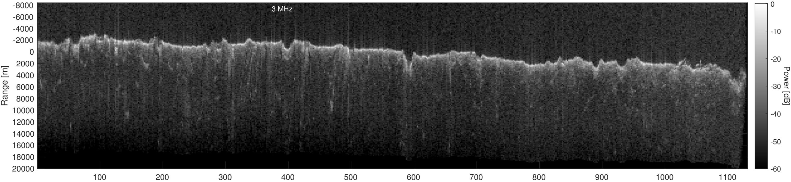
Orbit 20781, Depth-Corrected Cluttergram
