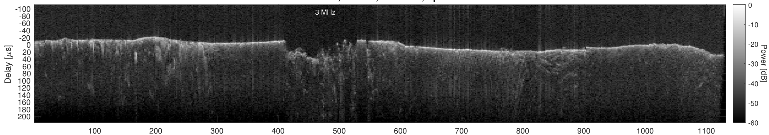
Orbit 20782, Cluttergram
