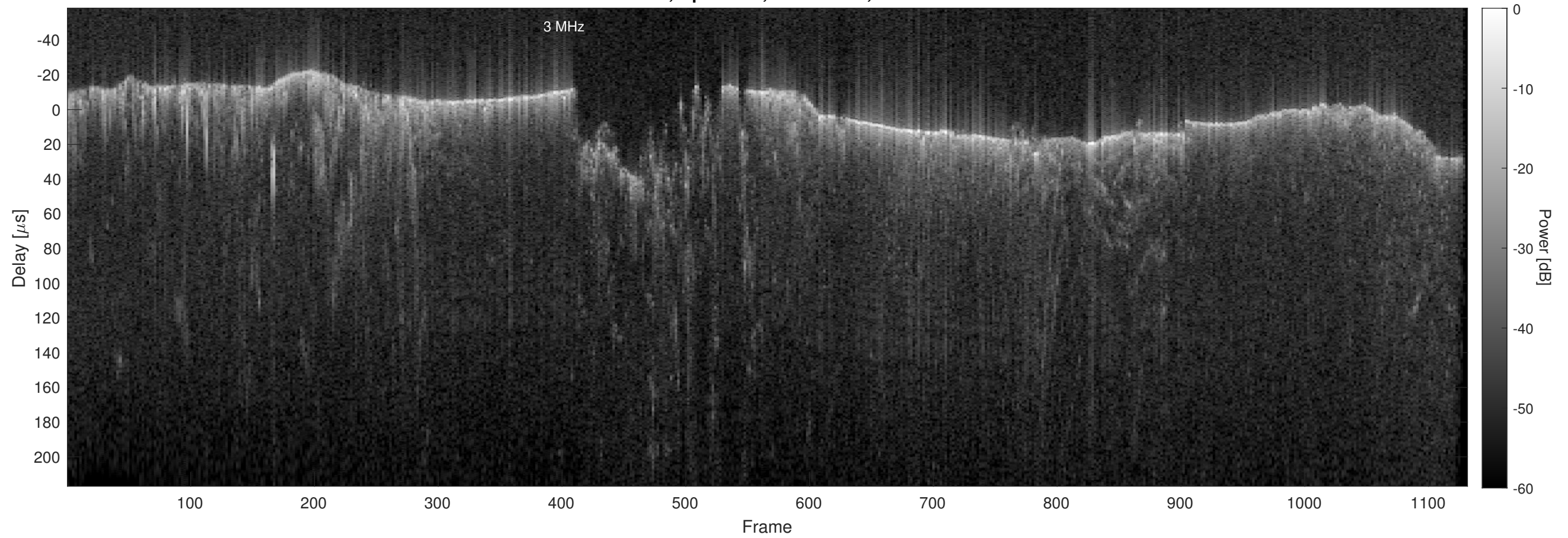
Orbit 20782, Optimized, No Window, Channel 2
