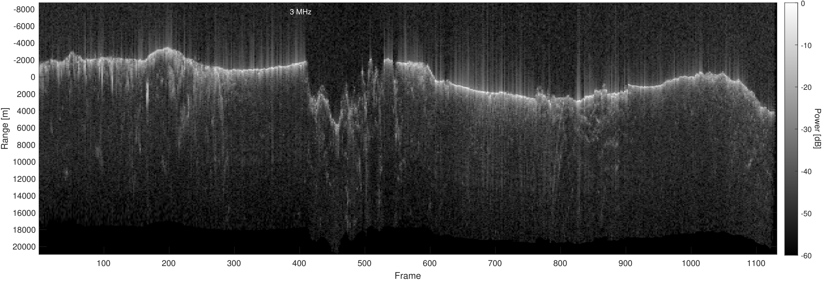
Orbit 20782, Optimized, No Window, Depth-Corrected, Channel 2
