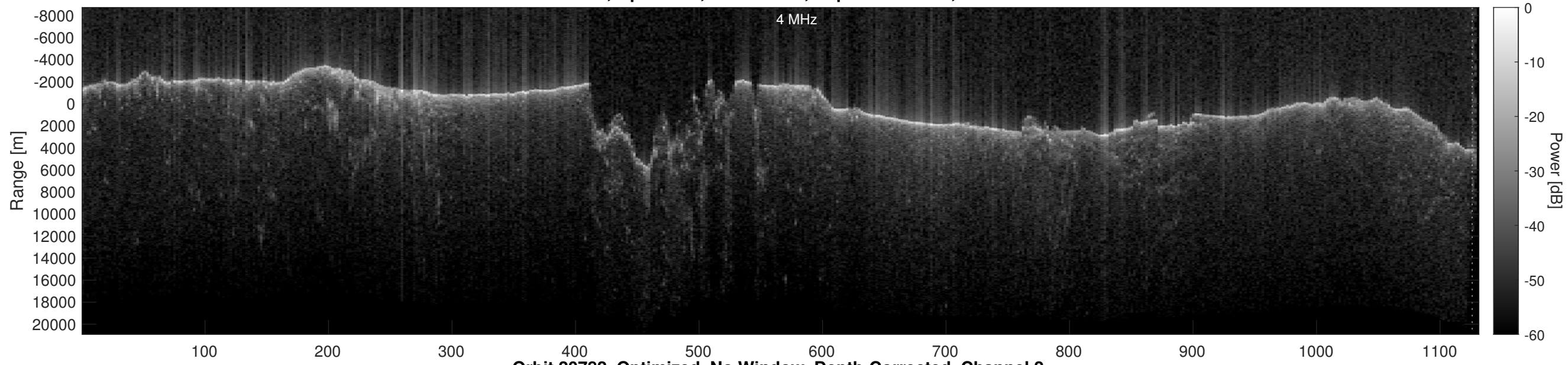
Orbit 20782, Optimized, No Window, Depth-Corrected, Channel 2
