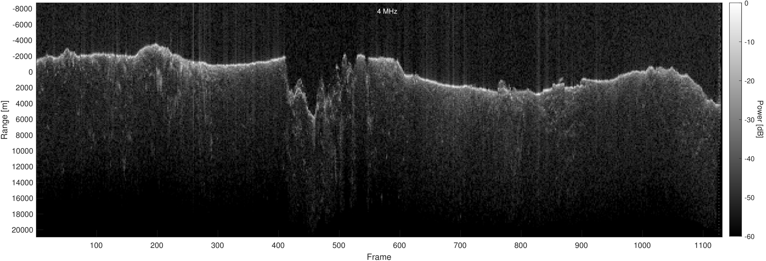
Orbit 20782, Optimized, Window, Depth-Corrected, Channel 2
