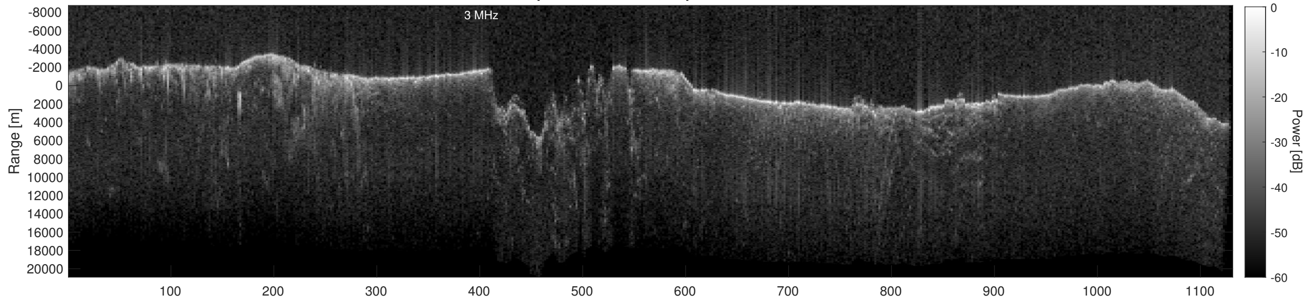
Orbit 20782, Depth-Corrected Cluttergram
