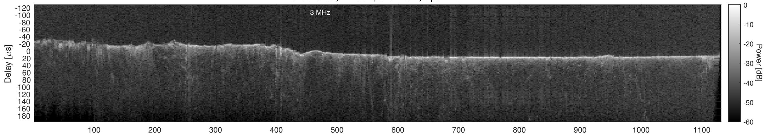
Orbit 20783, Cluttergram
