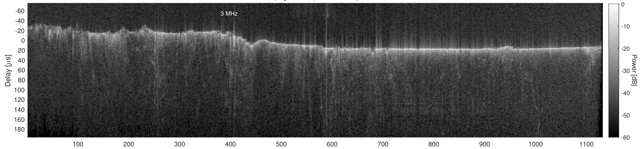
Orbit 20783, Cluttergram
