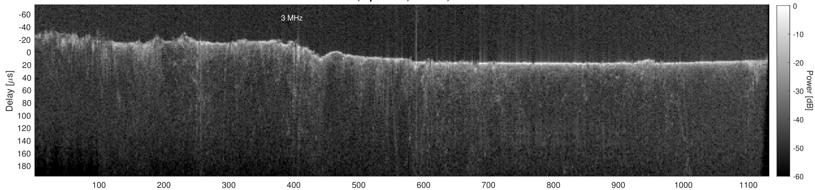
Orbit 20783, Cluttergram
