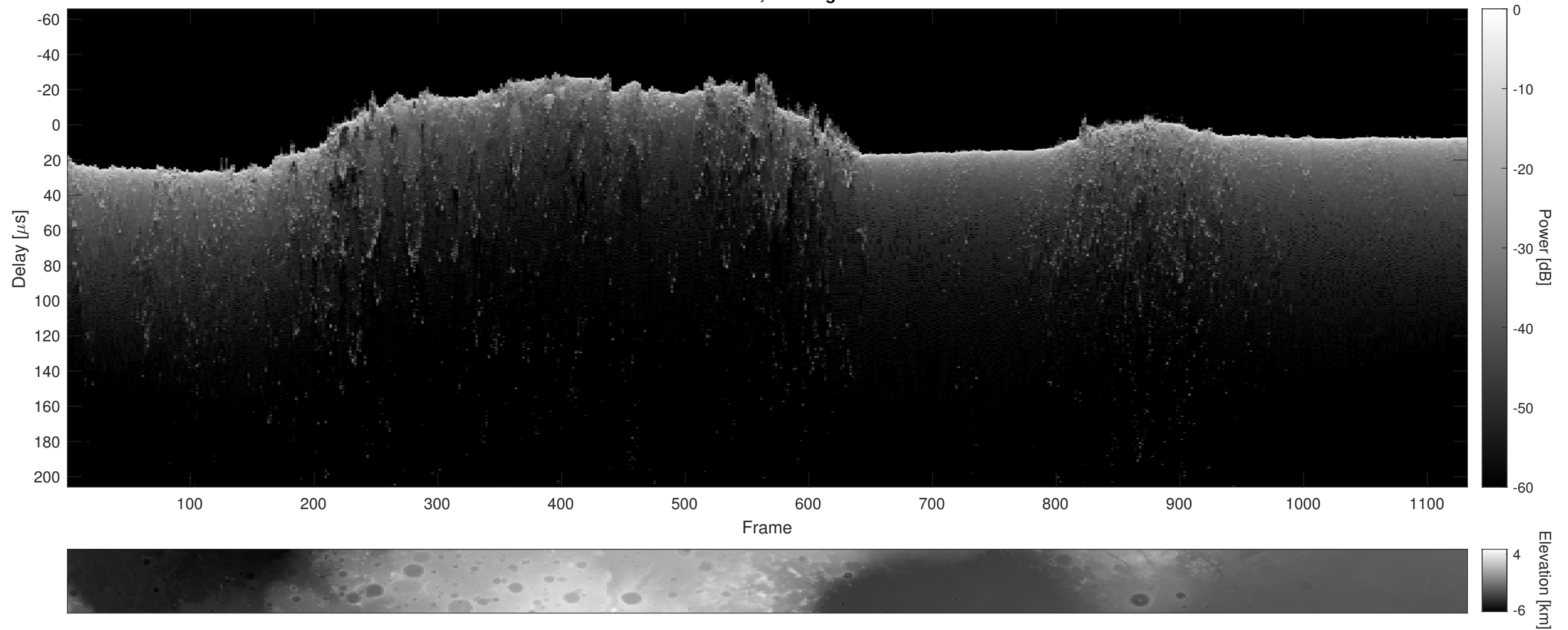
Orbit 20784, Cluttergram
