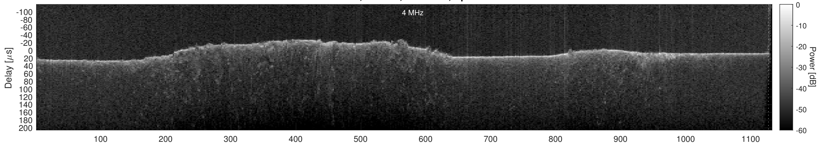
Orbit 20784, Cluttergram
