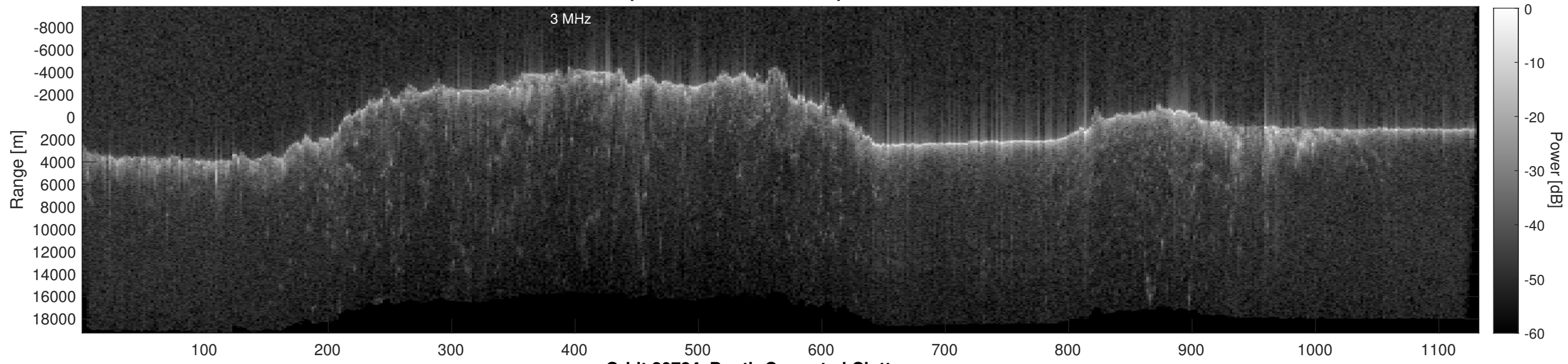
Orbit 20784, Depth-Corrected Cluttergram
