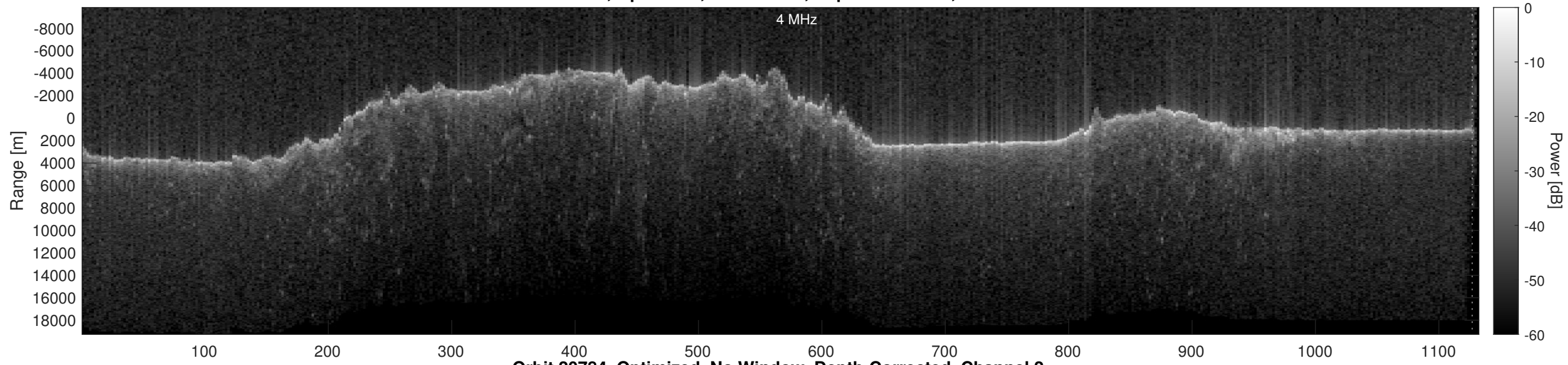
Orbit 20784, Optimized, No Window, Depth-Corrected, Channel 2
