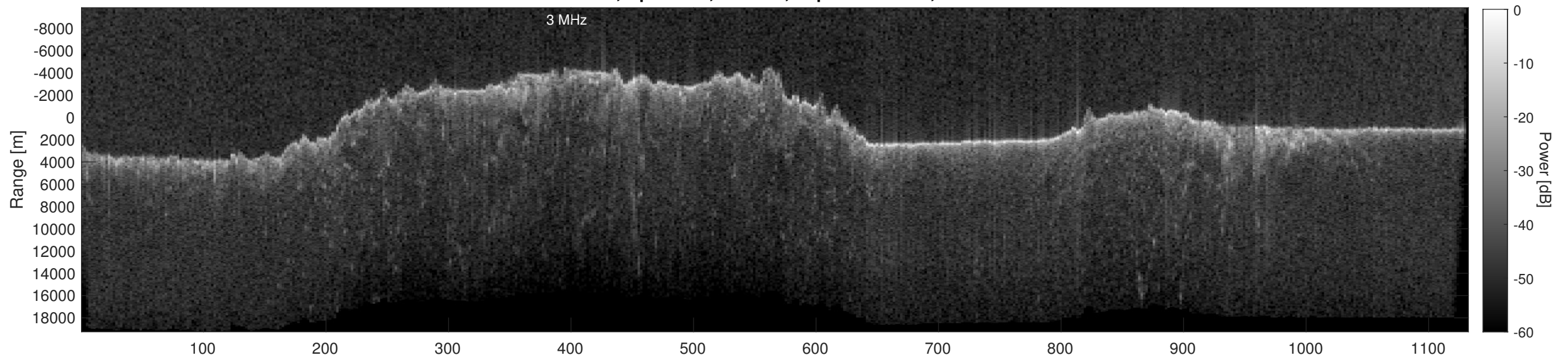
Orbit 20784, Depth-Corrected Cluttergram
