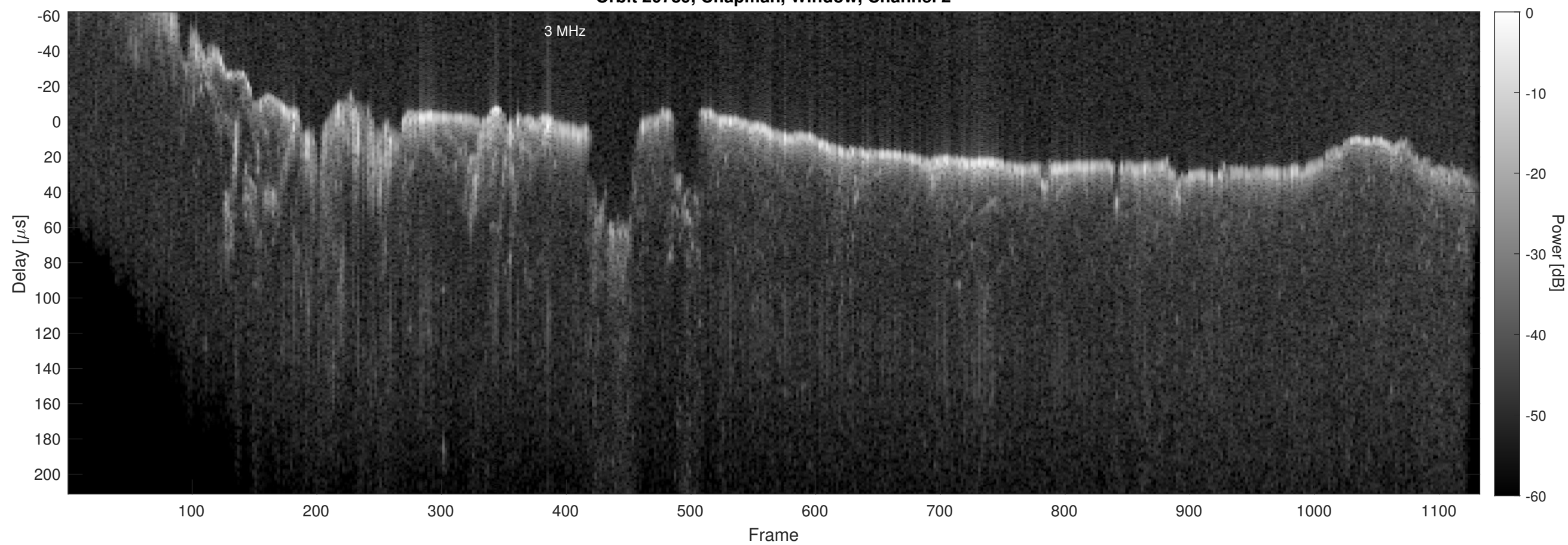
Orbit 20789, Chapman, Window, Channel 2
