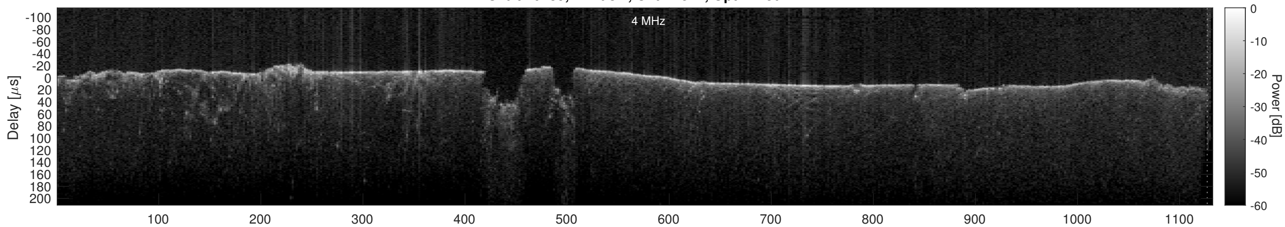
Orbit 20789, Cluttergram
