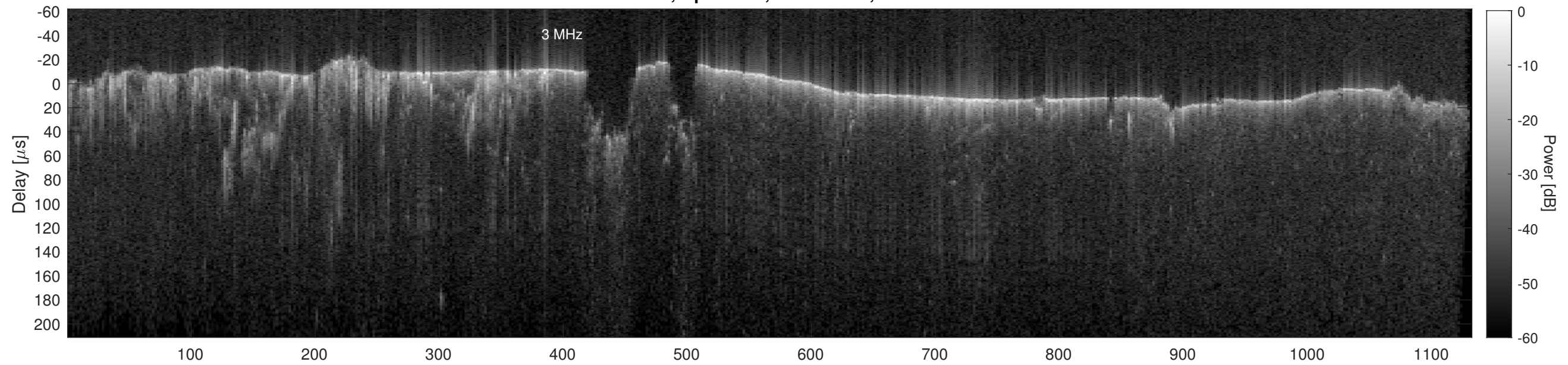
Orbit 20789, Cluttergram
