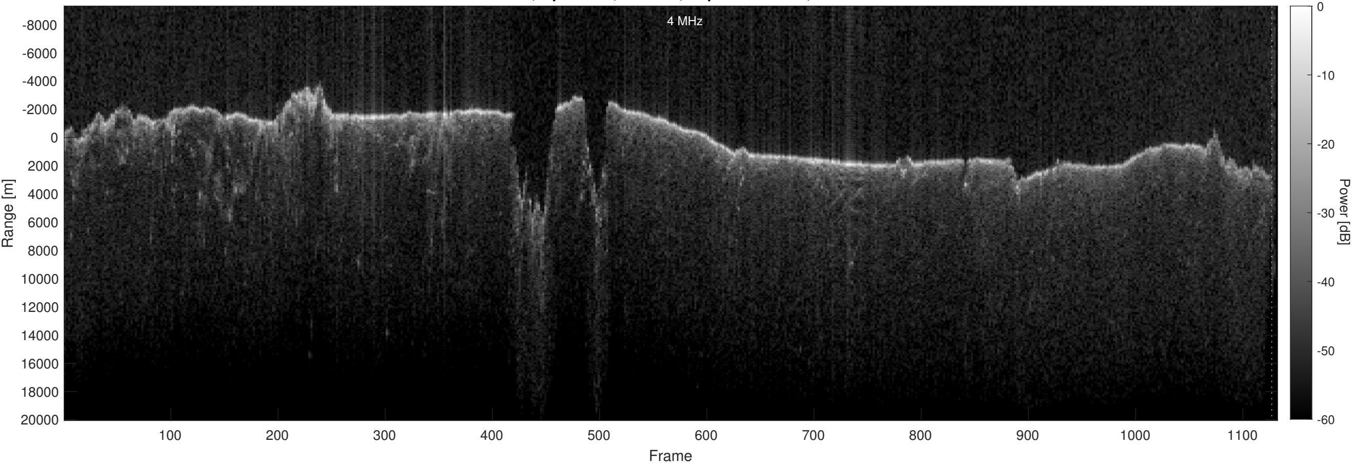
Orbit 20789, Optimized, Window, Depth-Corrected, Channel 2
