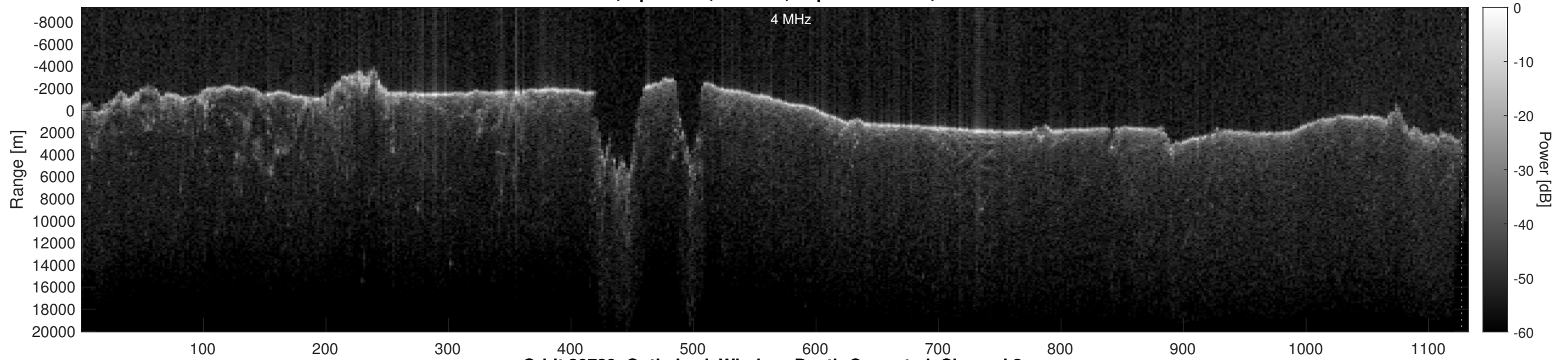
Orbit 20789, Optimized, Window, Depth-Corrected, Channel 2
