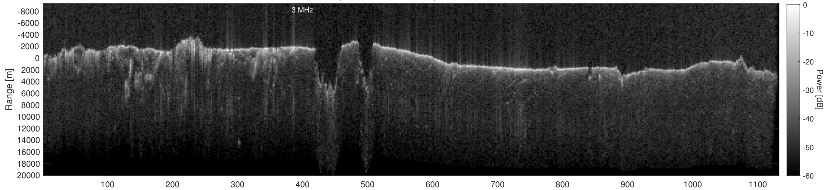
Orbit 20789, Depth-Corrected Cluttergram
