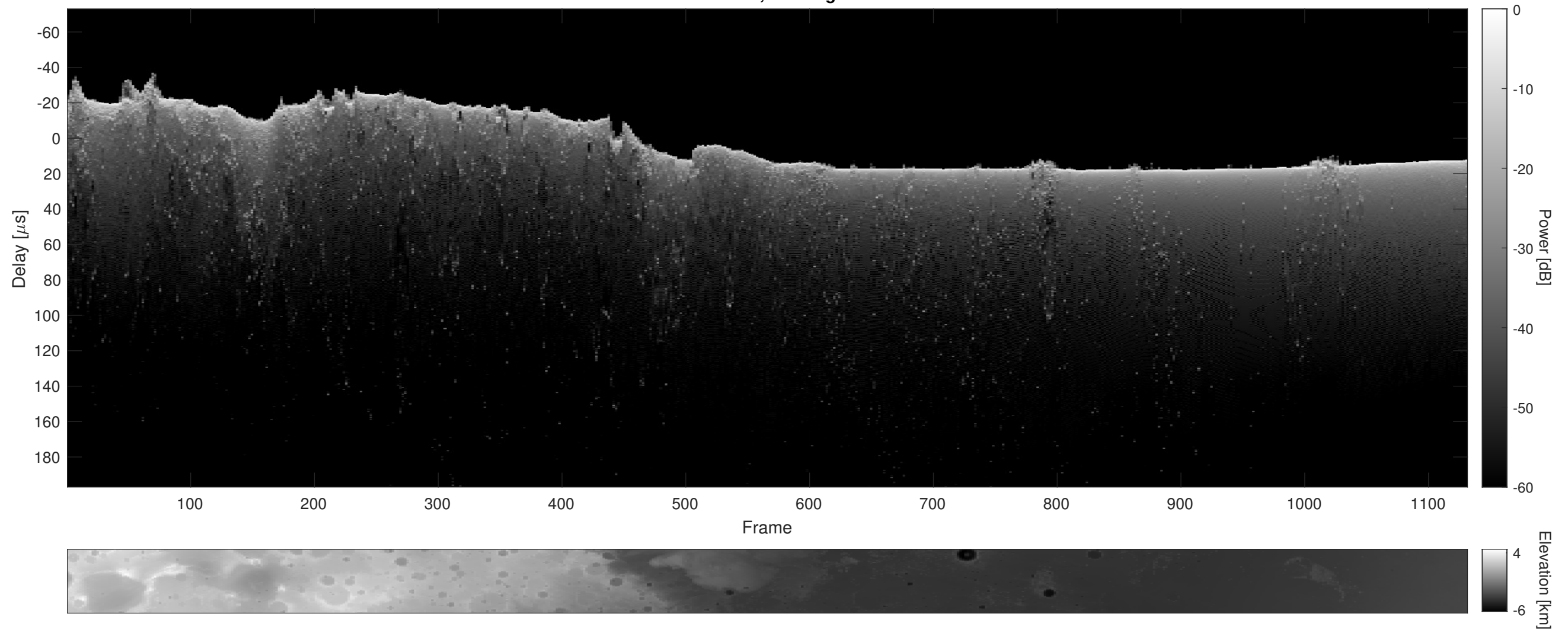
Orbit 20790, Cluttergram
