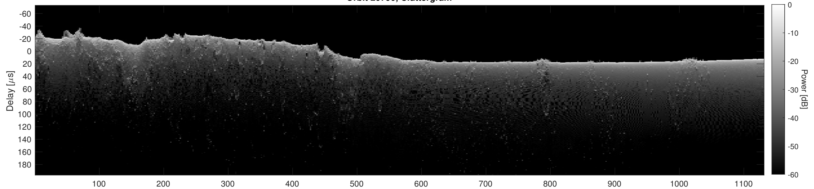
Orbit 20790, Cluttergram
