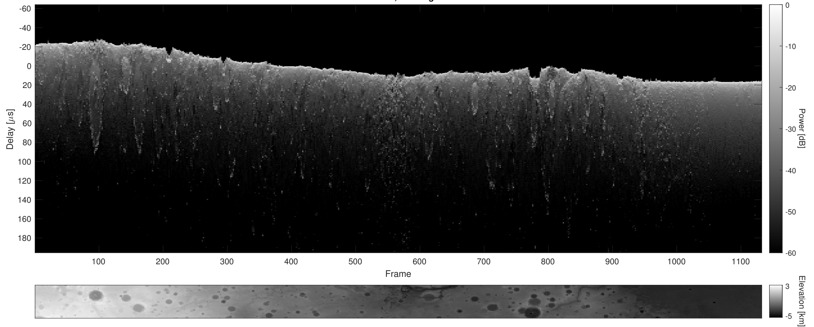
Orbit 20792, Cluttergram
