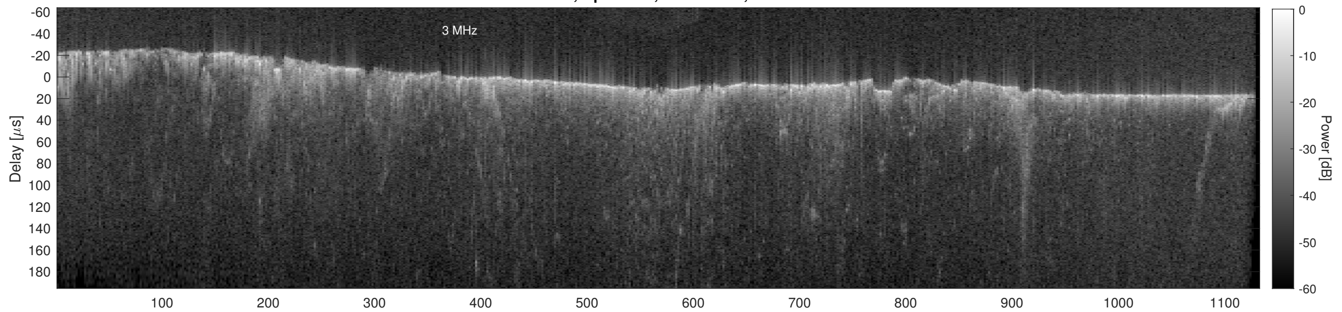
Orbit 20792, Cluttergram
