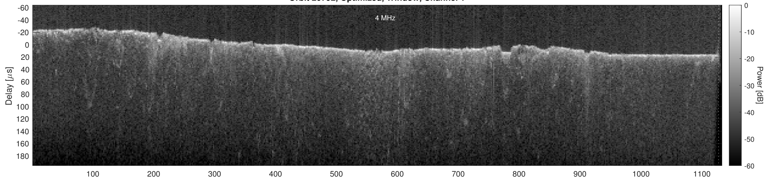
Orbit 20792, Optimized, Window, Channel 2
