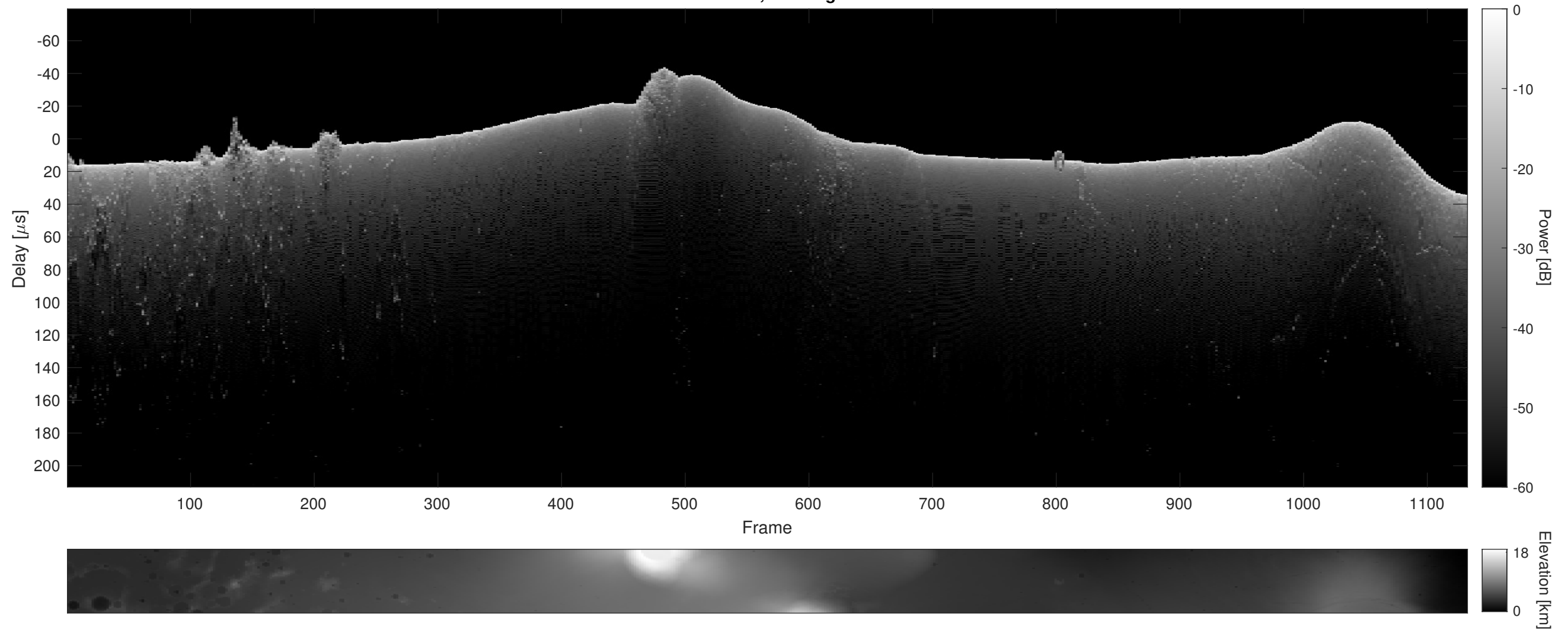
Orbit 20793, Cluttergram
