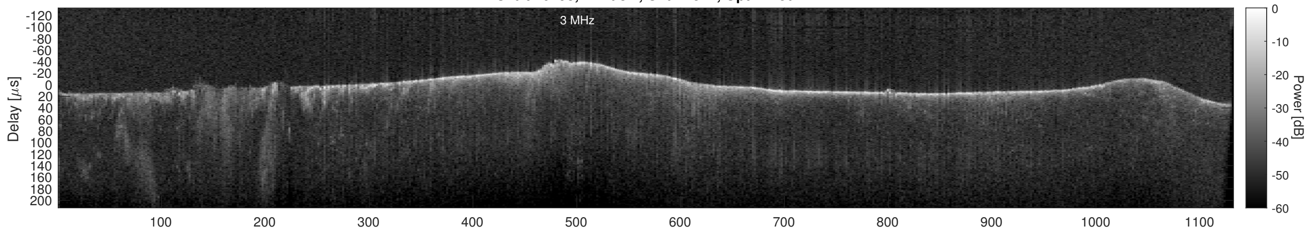
Orbit 20793, Cluttergram
