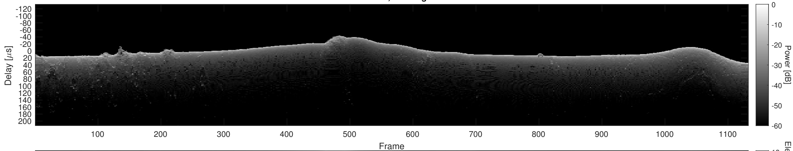
Orbit 20793, Cluttergram
