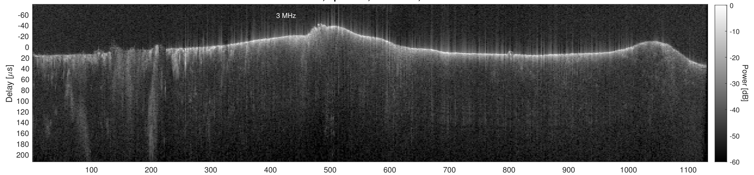
Orbit 20793, Cluttergram
