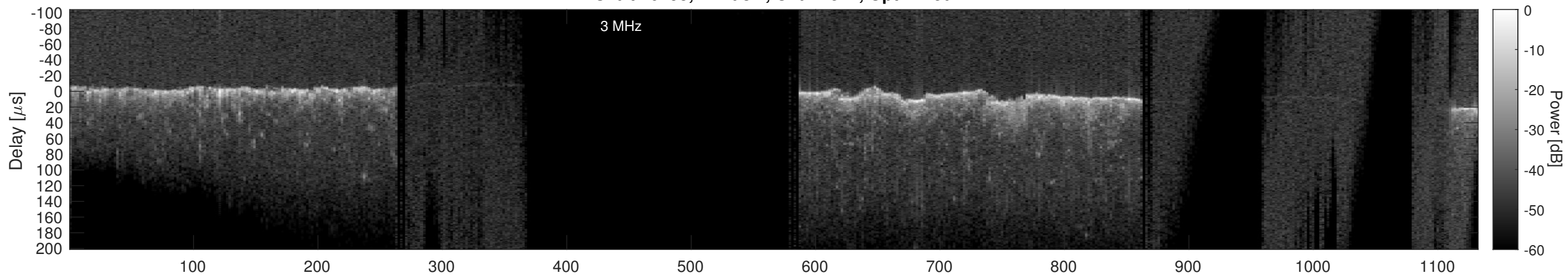
Orbit 20795, Cluttergram
