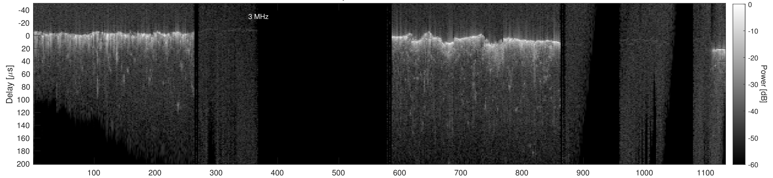
Orbit 20795, Cluttergram
