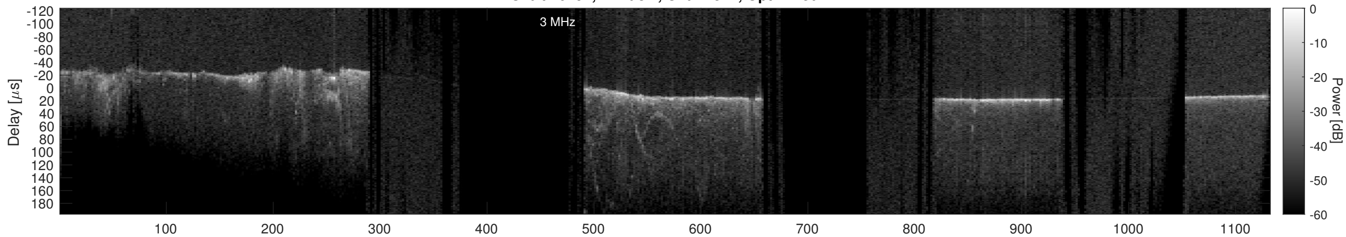
Orbit 20797, Cluttergram
