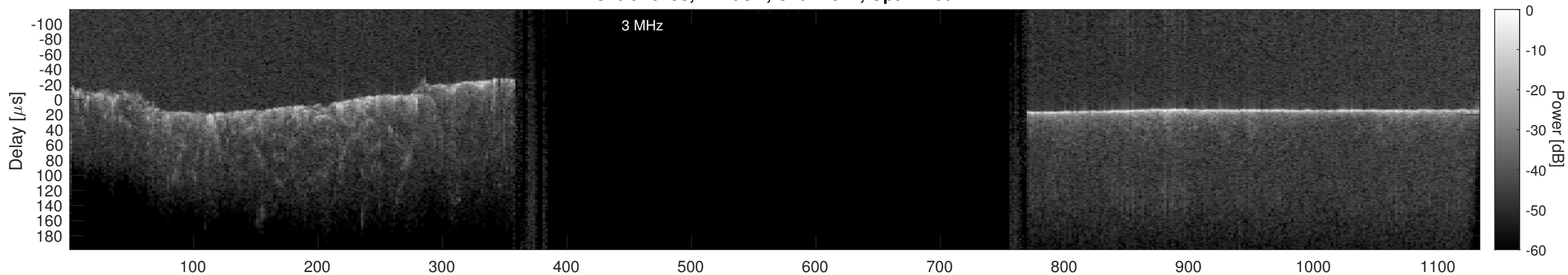
Orbit 20798, Cluttergram
