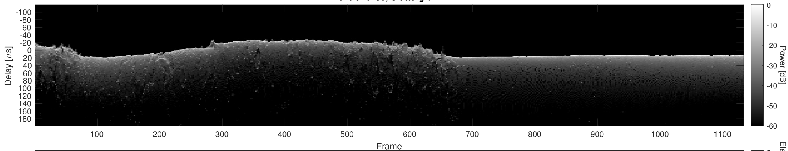
Orbit 20798, Cluttergram
