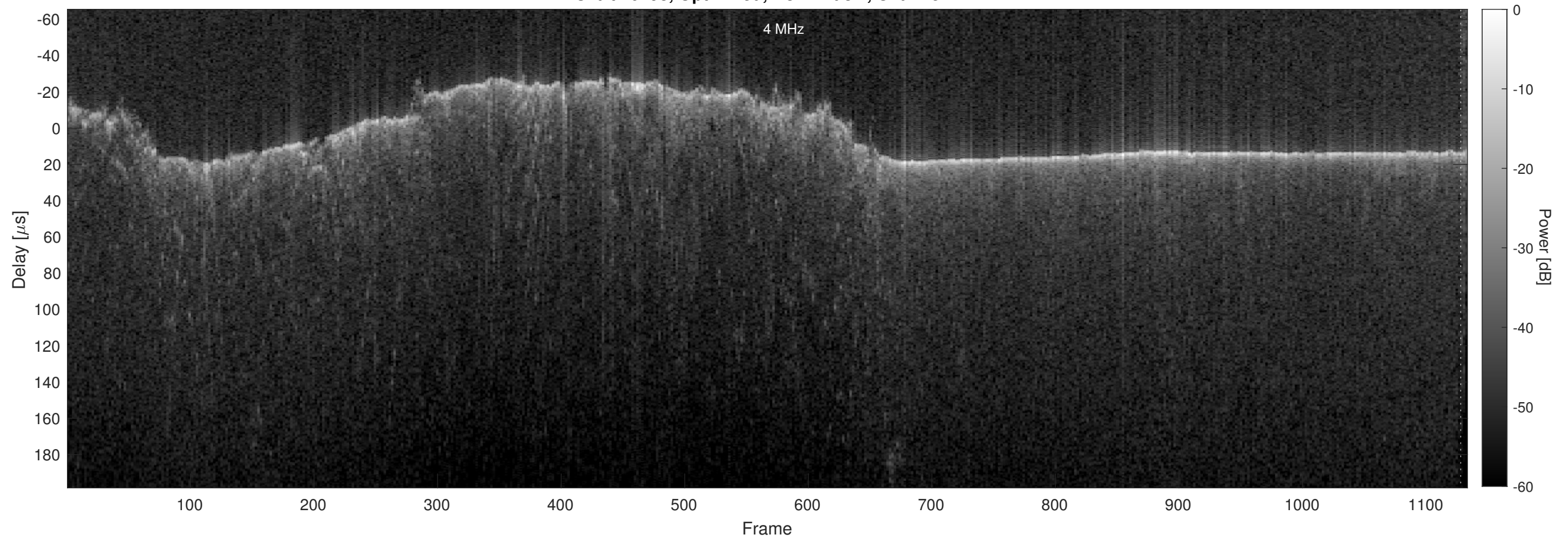
Orbit 20798, Optimized, No Window, Channel 2
