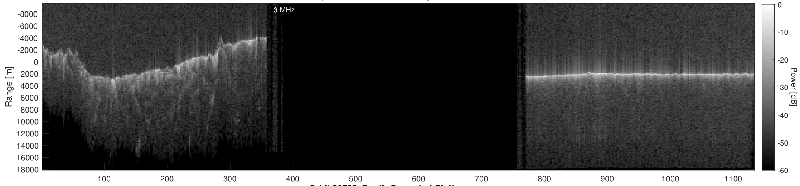
Orbit 20798, Depth-Corrected Cluttergram
