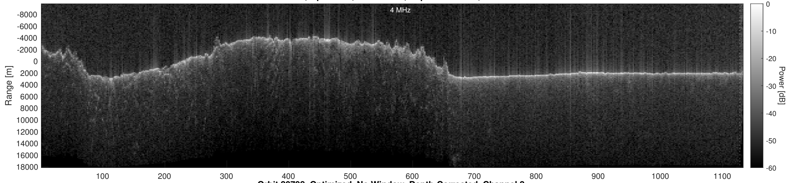
Orbit 20798, Optimized, No Window, Depth-Corrected, Channel 2
