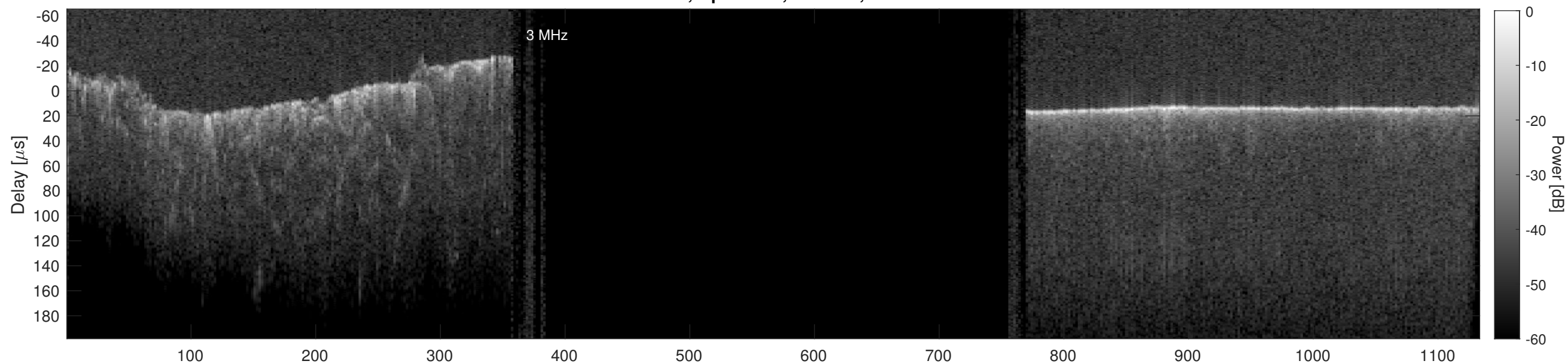
Orbit 20798, Cluttergram
