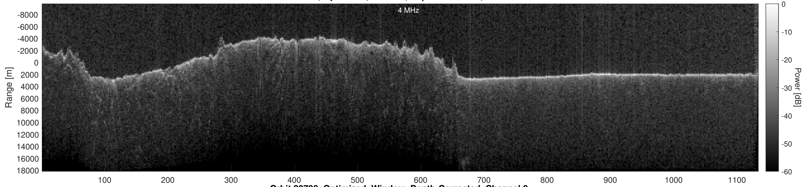
Orbit 20798, Optimized, Window, Depth-Corrected, Channel 2
