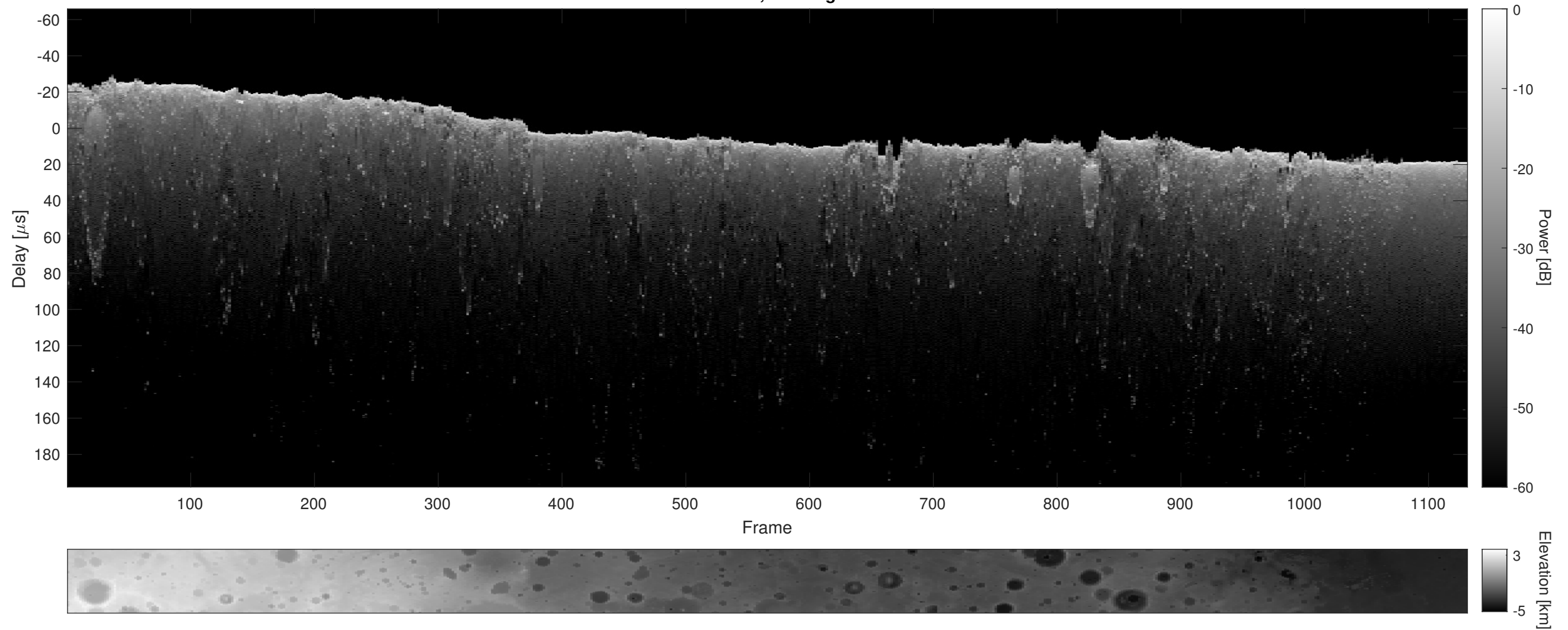
Orbit 20799, Cluttergram
