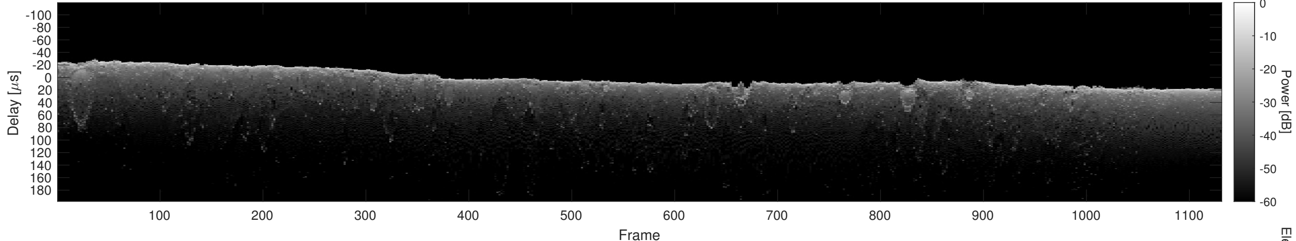
Orbit 20799, Cluttergram
