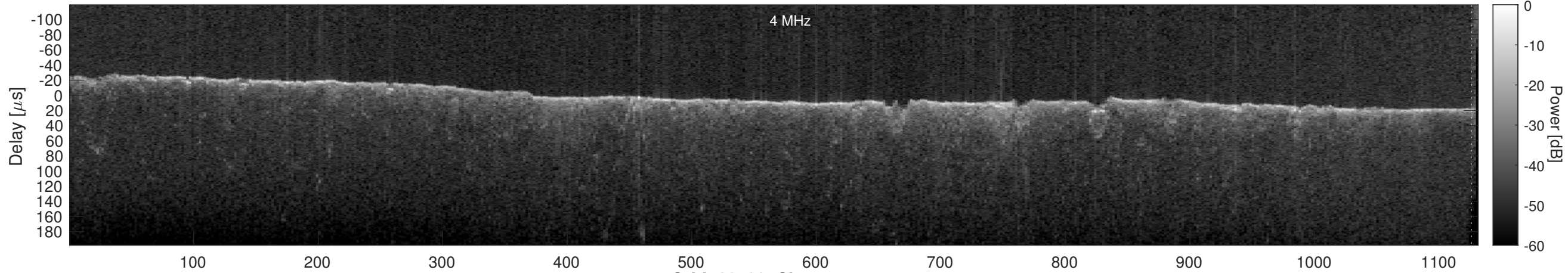
Orbit 20799, Cluttergram
