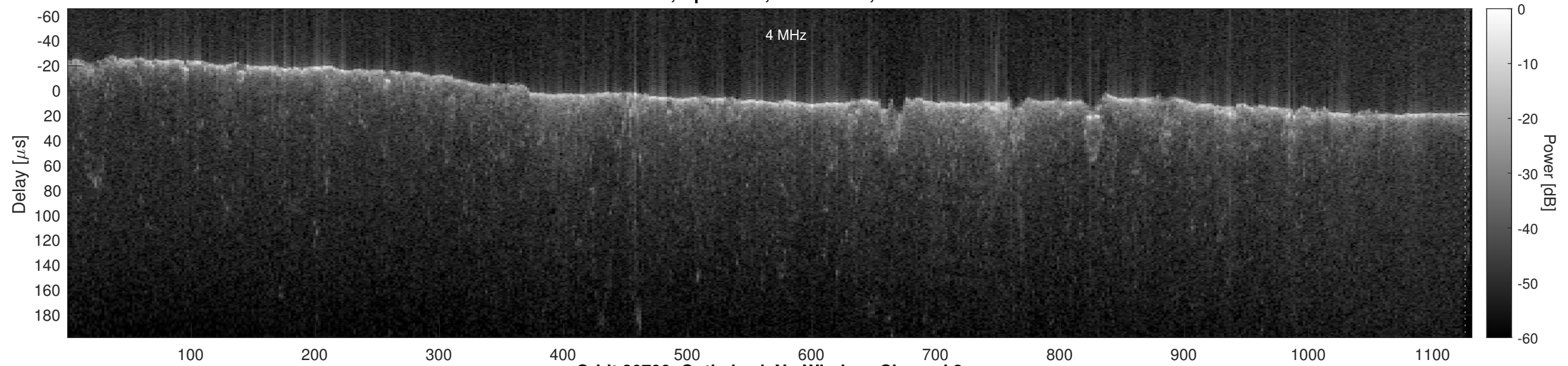
Orbit 20799, Optimized, No Window, Channel 2
