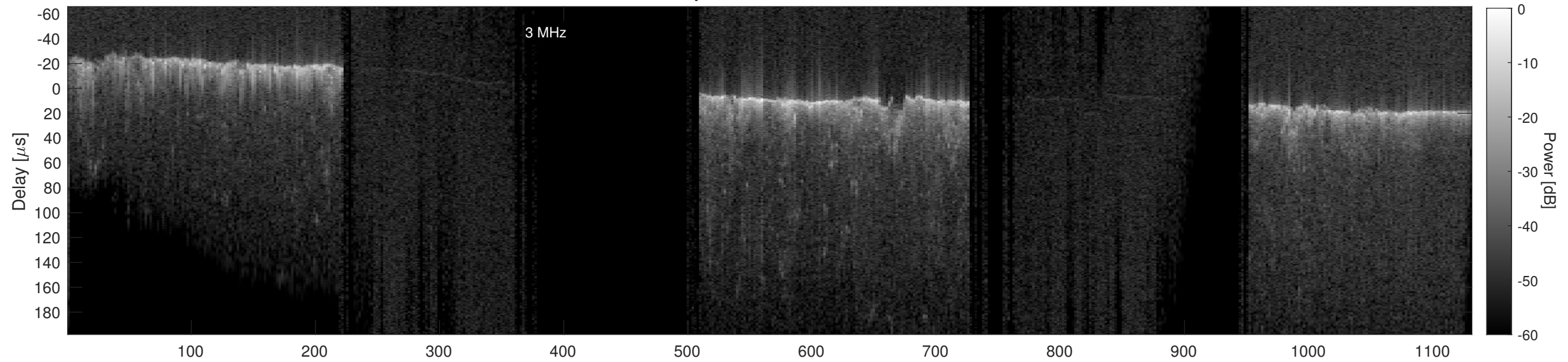
Orbit 20799, Cluttergram
