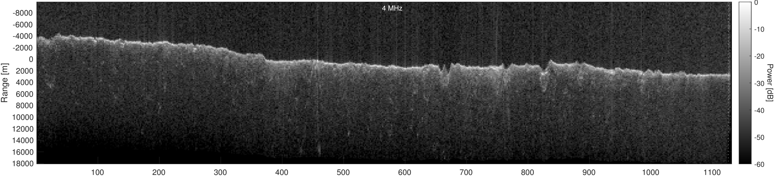
Orbit 20799, Optimized, Window, Depth-Corrected, Channel 2
