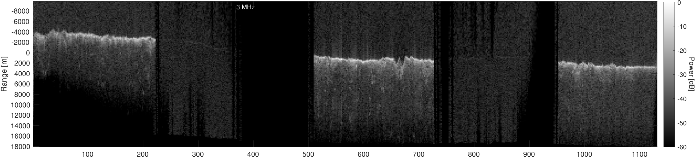
Orbit 20799, Depth-Corrected Cluttergram
