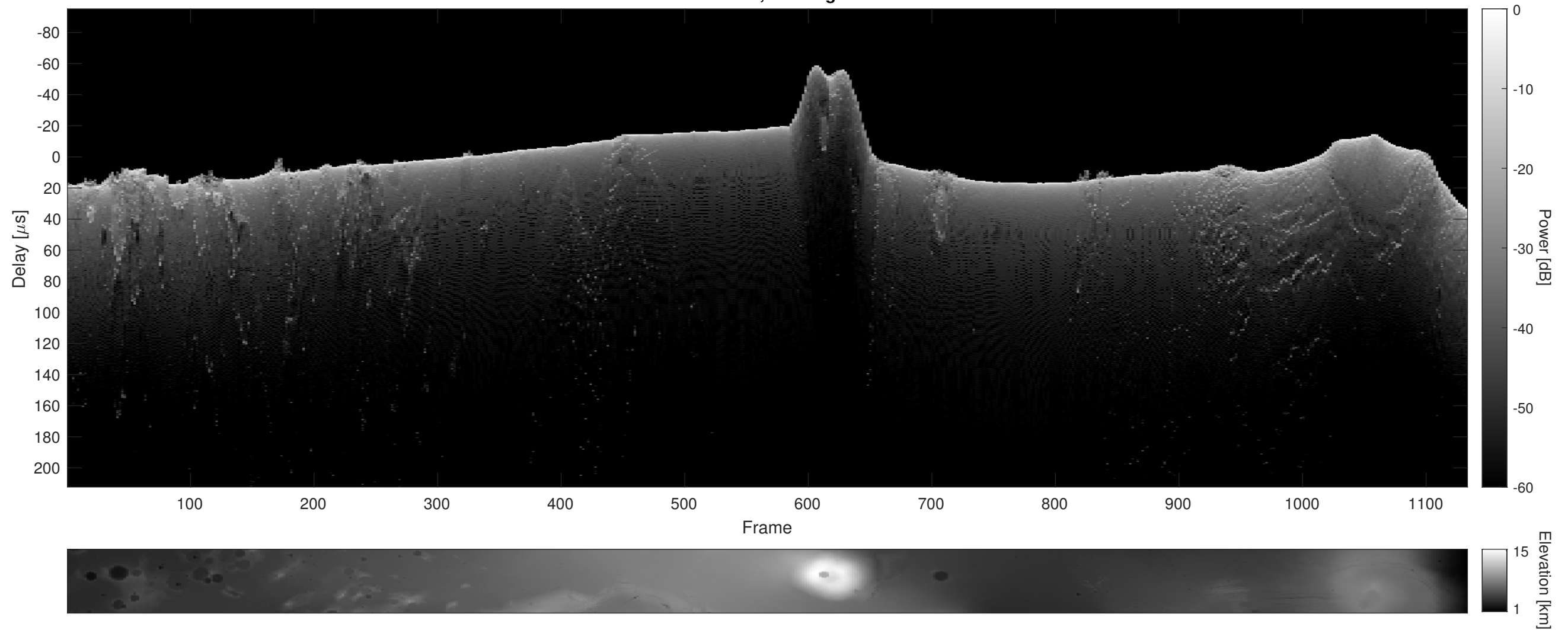
Orbit 20800, Cluttergram
