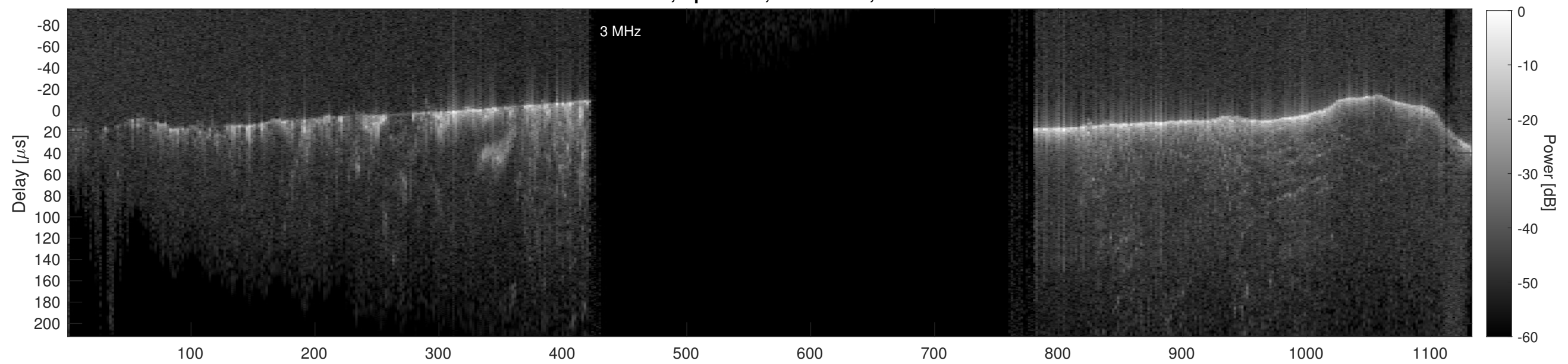
Orbit 20800, Cluttergram
