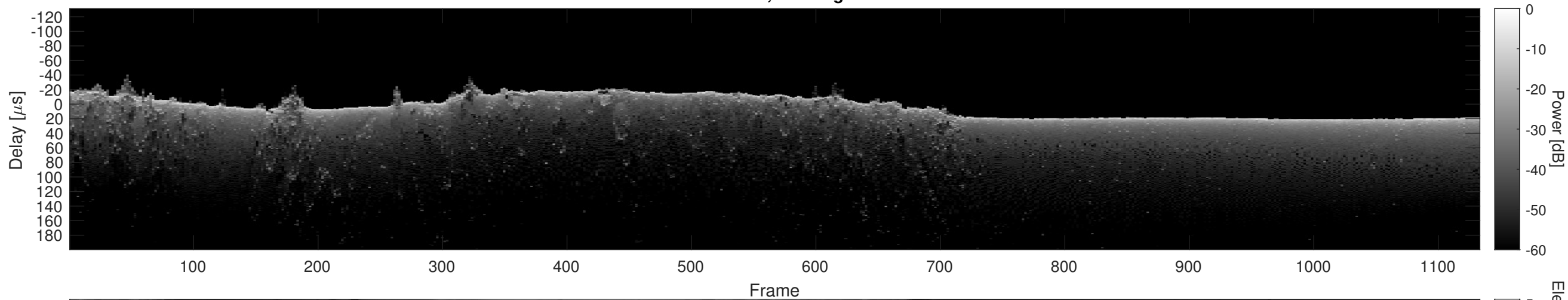
Orbit 20805, Cluttergram
