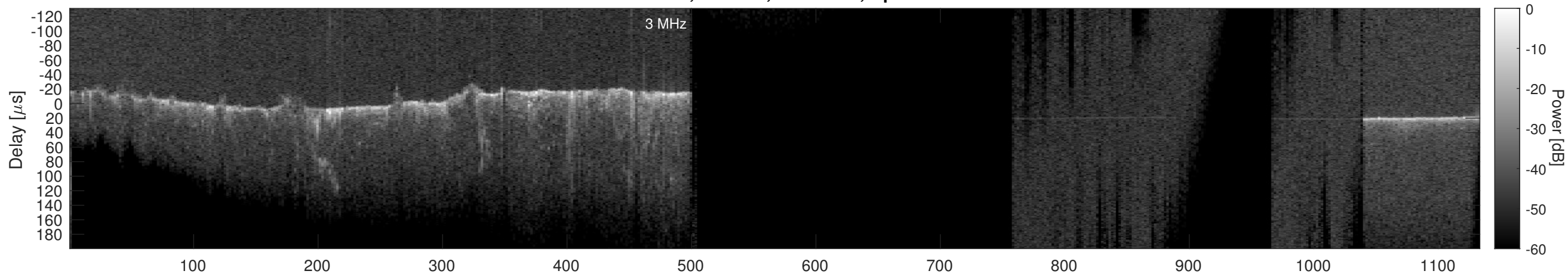
Orbit 20805, Cluttergram
