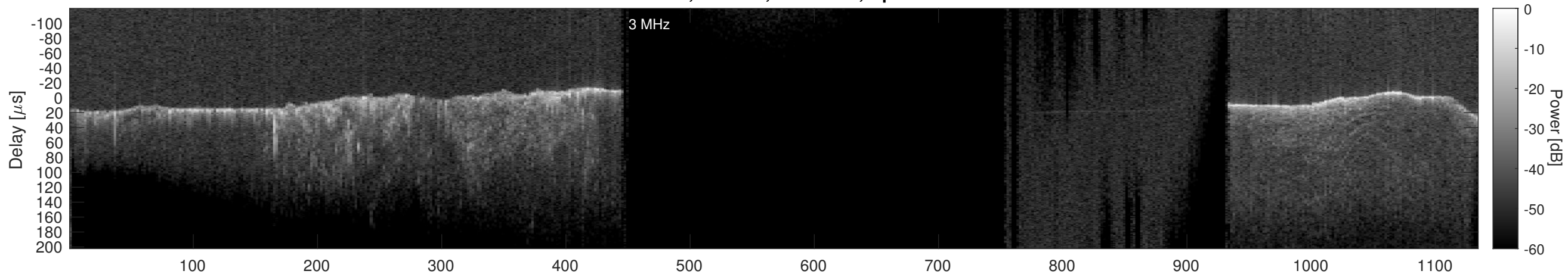
Orbit 20807, Cluttergram
