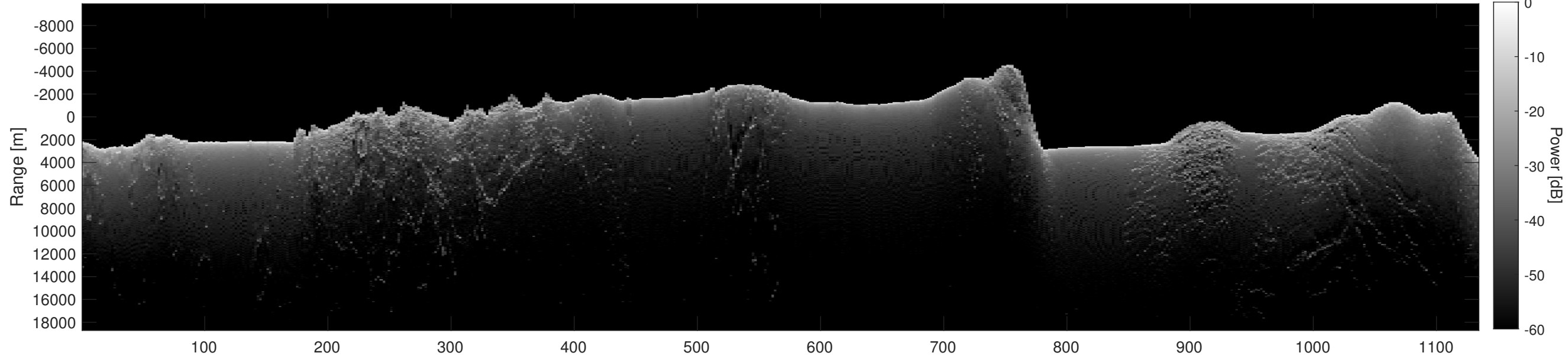
Orbit 20807, Depth-Corrected Cluttergram
