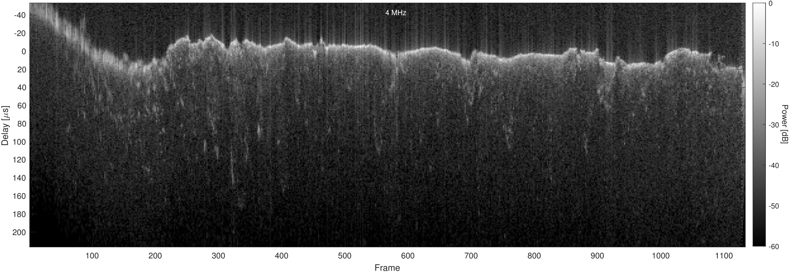
Orbit 20809, Chapman, No Window, Channel 2
