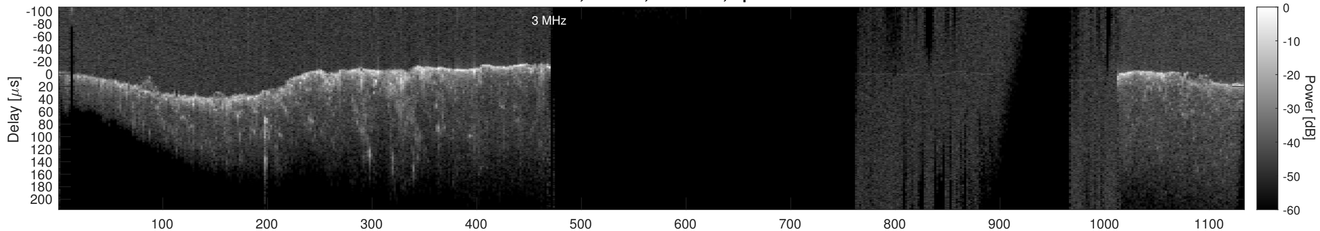
Orbit 20809, Cluttergram
