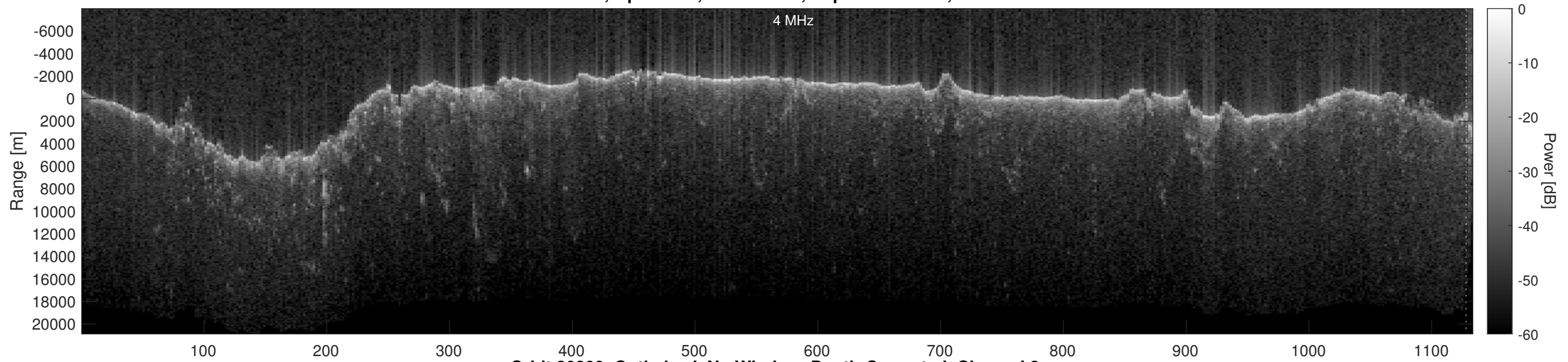
Orbit 20809, Optimized, No Window, Depth-Corrected, Channel 2
