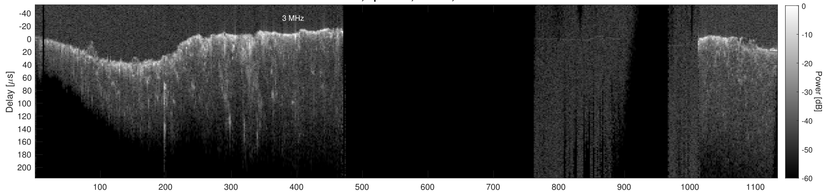
Orbit 20809, Cluttergram
